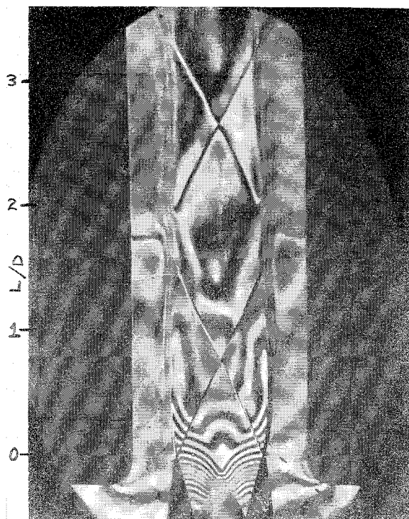
Fig. 2 Mixer interferogram.
