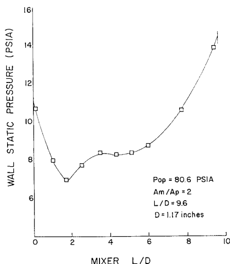
Fig. 1 Mixer wall static pressure profile.
